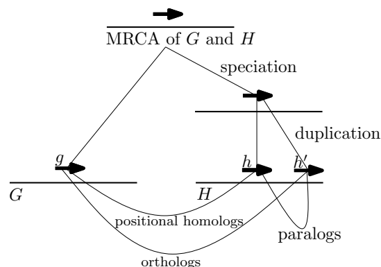
Fig. 1. The gene tree for three genes g , h , and h' that descended from a single ancestral gene in the most recent common ancestor (MRCA) of genome G and H . Gene g is orthologous to both h and h' , but only g and h are positional homologs because h is the original gene that was duplicated to get h' . Genes h and h' are paralogs as they are separated by a duplication event.
