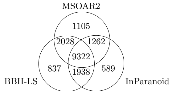
Fig. 7. Venn diagram showing the overlap between the true positives reported by BBH-LS, MSOAR2, and InParanoid for the human-mouse dataset.
