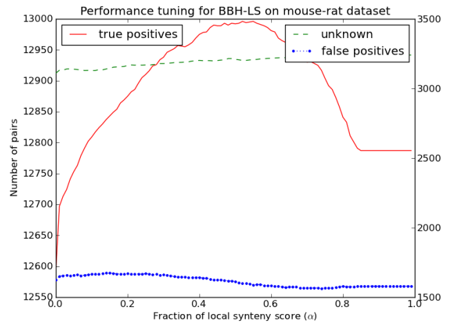
Fig. 5. Performance of BBH-LS for different weightage of gene context similarity to sequence similarity on the mouse-rat dataset. Left axis indicates the number of pairs of true positives and the right axis indicate the number of unknown pairs and false positives.
