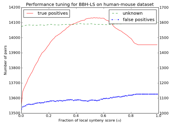
Fig. 4. Performance of BBH-LS for different weightage of gene context similarity to sequence similarity on the human-mouse dataset. Left axis indicates the number of pairs of true positives and the right axis indicate the number of unknown pairs and false positives.
