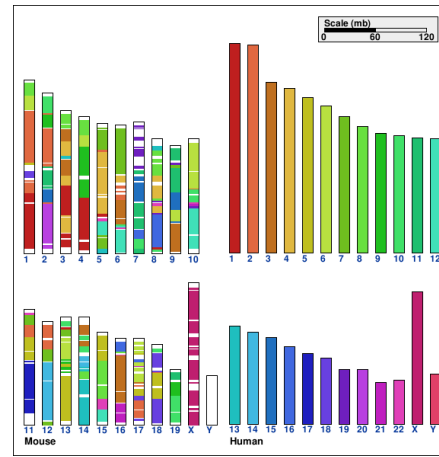
Fig. 2. Conserved synteny blocks between human and mouse genome generated by the Cinteny web server [19]
