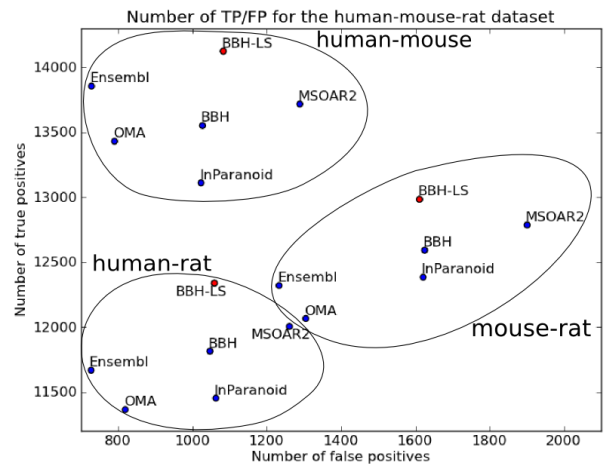
Fig. 6. Plot of number of true positives vs number of false positives in the output of BBH-LS, BBH, MSOAR2, InParanoid, OMA, and Ensembl Compara for the human-mouse, human-rat, and mouse-rat dataset
